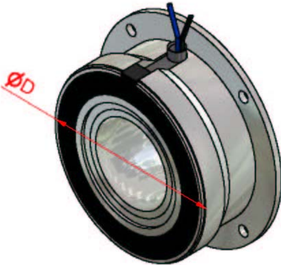
Stator for brakes
